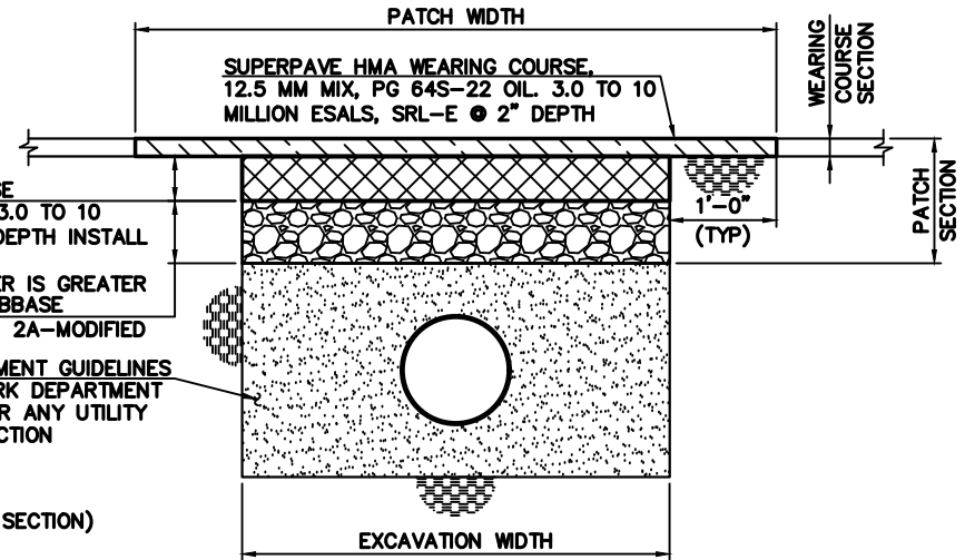
PATCH TYPICAL SECTION
