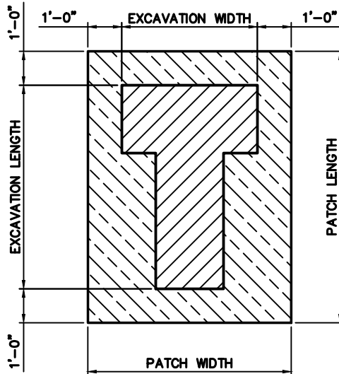
NON RECTANGULAR CUT PATCH
