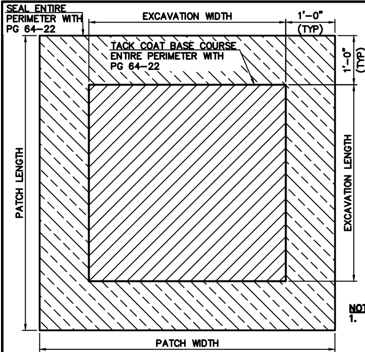
PATCH PLAN VIEW
